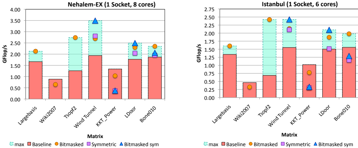
Fig. 12: Parallel performance of SpMV kernels on Nehalem-EX ( left ) and Istanbul ( right ). Baseline original CSB code is in red; circles show bitmasked register blocks; triangles and squares show symmetric algorithm with and without bitmasked register blocking, respectively; green shows overall performance gain of our approach. The first three matrices are unsymmetric, followed by four symmetric matrices. The unsymmetric algorithms (‘Baseline’ and ‘Bitmasked’) run on original matrices while the symmetric algorithms (‘Symmetric’ and ‘Bitmasked sym’) run on RCM ordered matrices.
